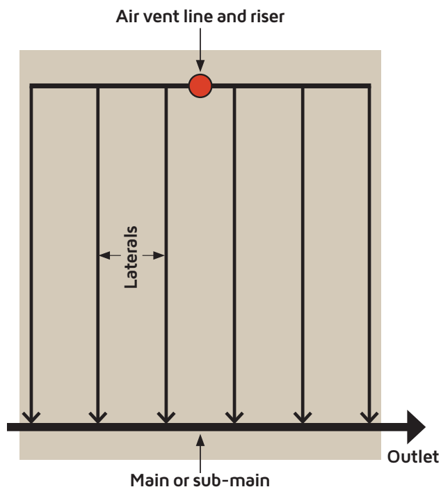
Figure 3. Overhead view of a tile drainage system including vent
